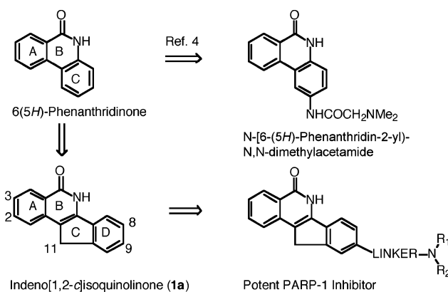
Figure 1. Design of novel PARP-1 inhibitors.
