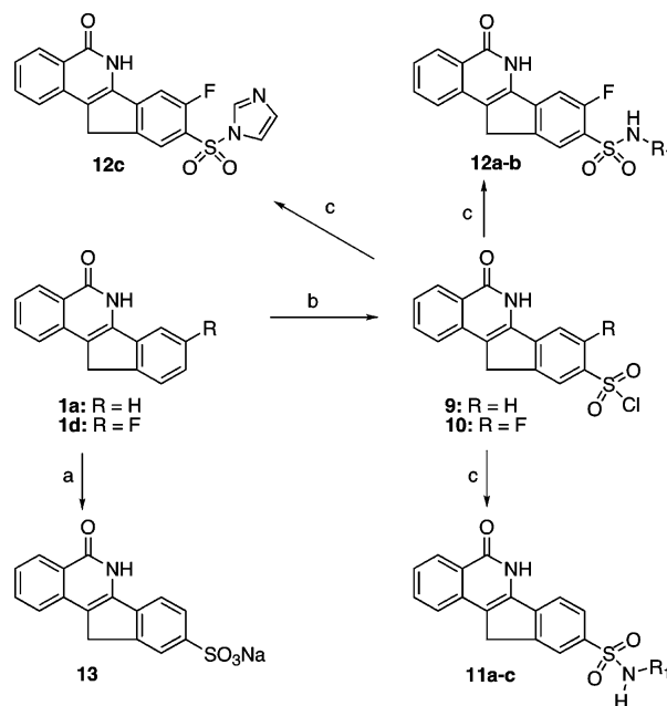
Scheme 3. Synthesis of C-9 Sulfonamide Derivatives of Indeno[1,2- c ]isoquinolinones a
