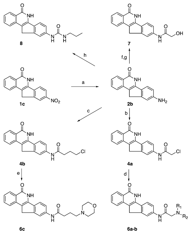
Scheme 2. Synthesis of C-9 Substituted Indeno[1,2- c ]isoquinolinones a
